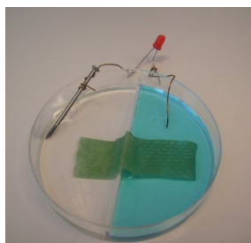
Figure 3: Daniell cell in a petri dish
