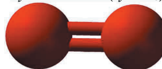
Dioxygen
