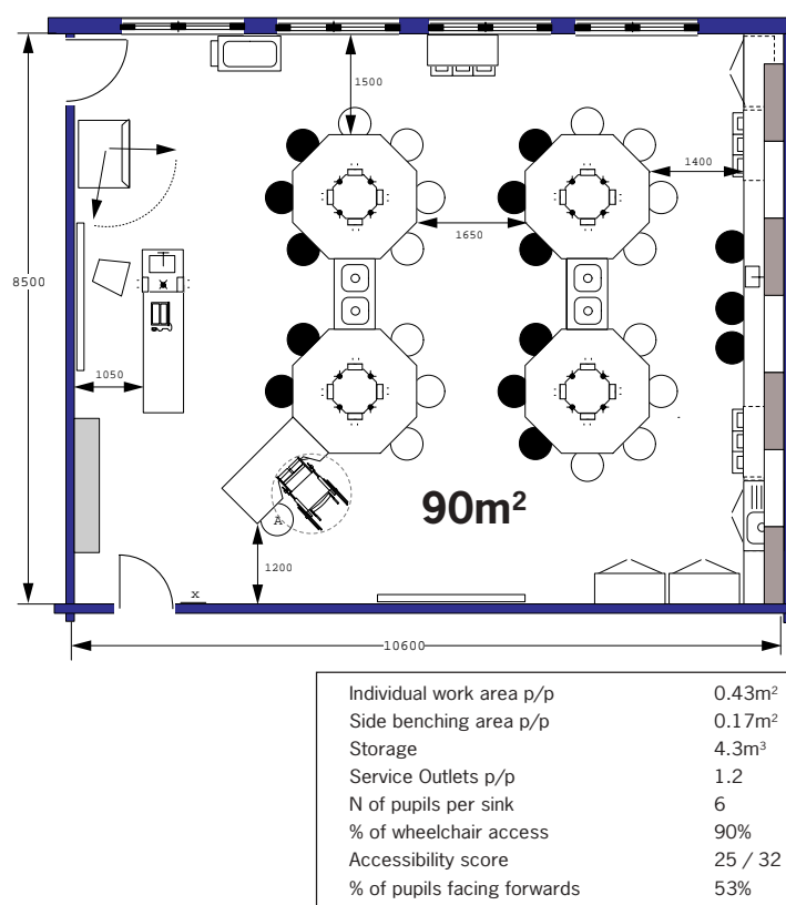
Figure 2/22a: Island Octagon (8.5m).
