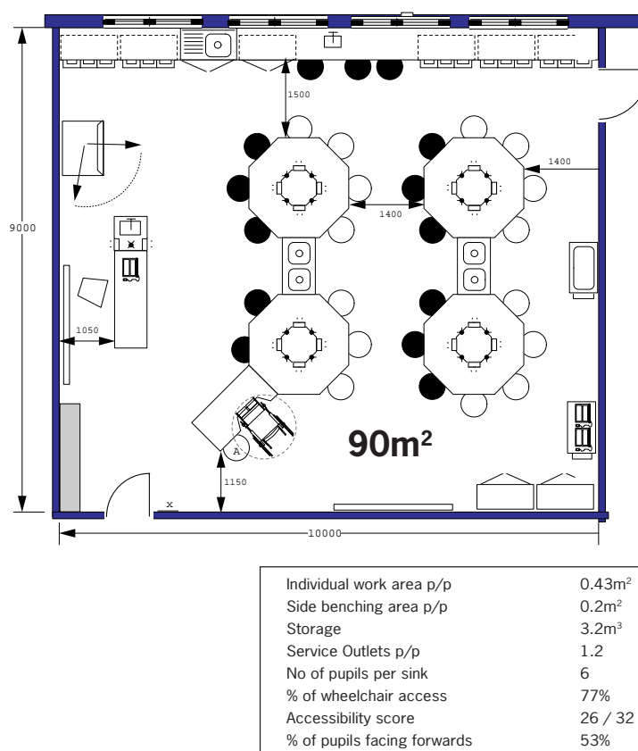
Figure 2/22b: Island Octagon (9m).
