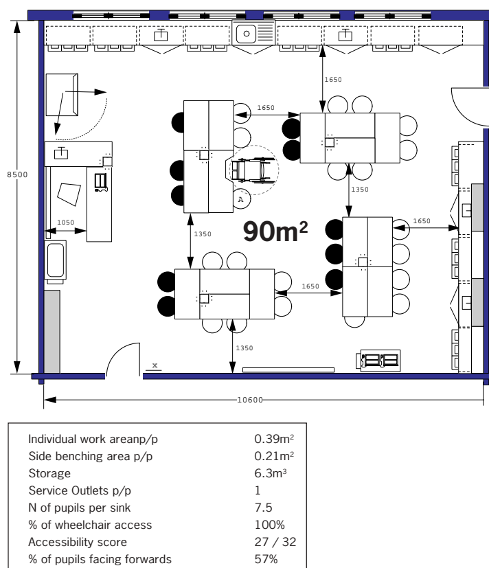
Figure 2/19a: Pod and Perimeter Sinks (8.5m).
