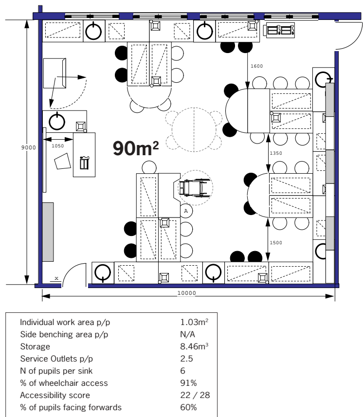
Figure 2/23b: Perimeter Serviced Tables (9m).
