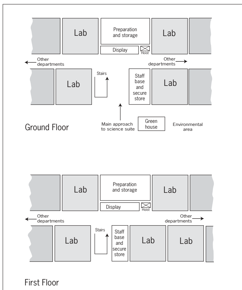
Figure 1/6 Linear On Two Floors
