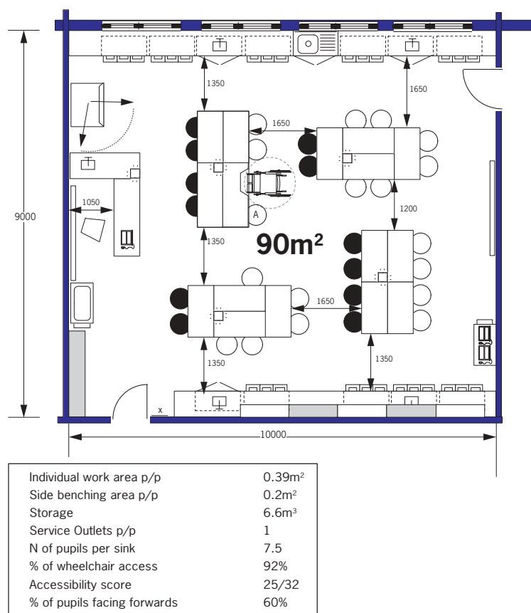
Figure 2/19b: Pod and Perimeter Sinks (9m).
