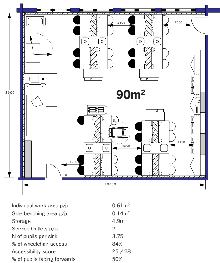
Figure 2/11b: Spine and Island Sink (9m).
