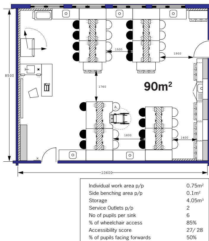
Figure 2/10a: Spine and Perimeter Sink (8.5m).
