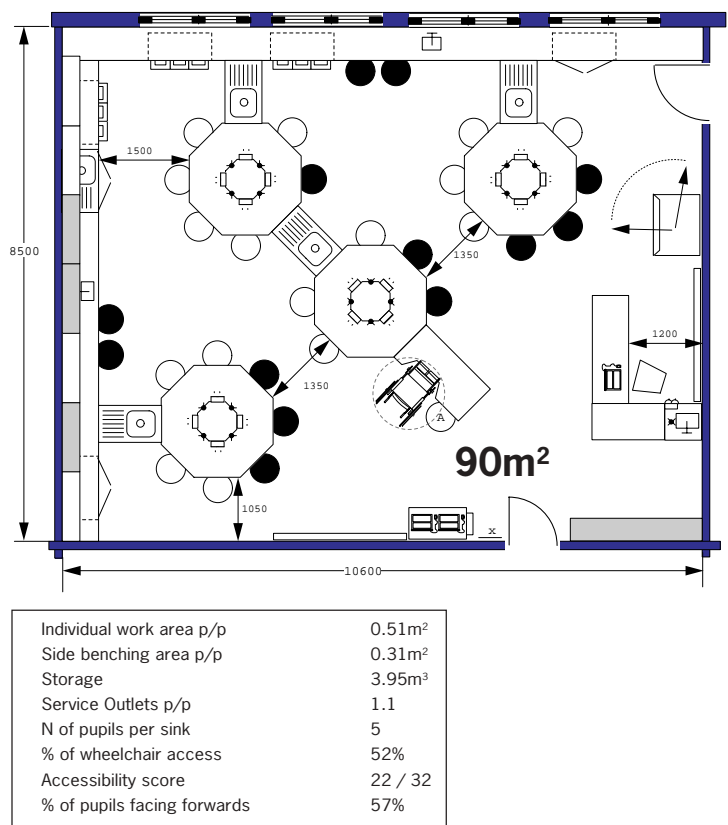
Figure 2/21a: Perimeter Serviced Octagon (8.5m).
