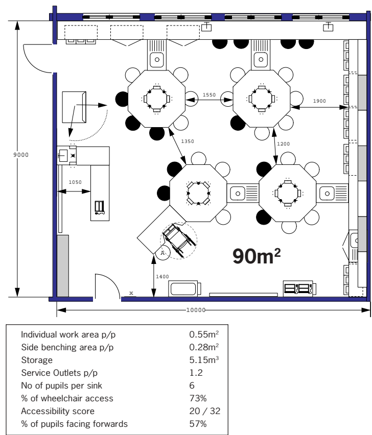
Figure 2/21b: Perimeter Serviced Octagon (9m).
