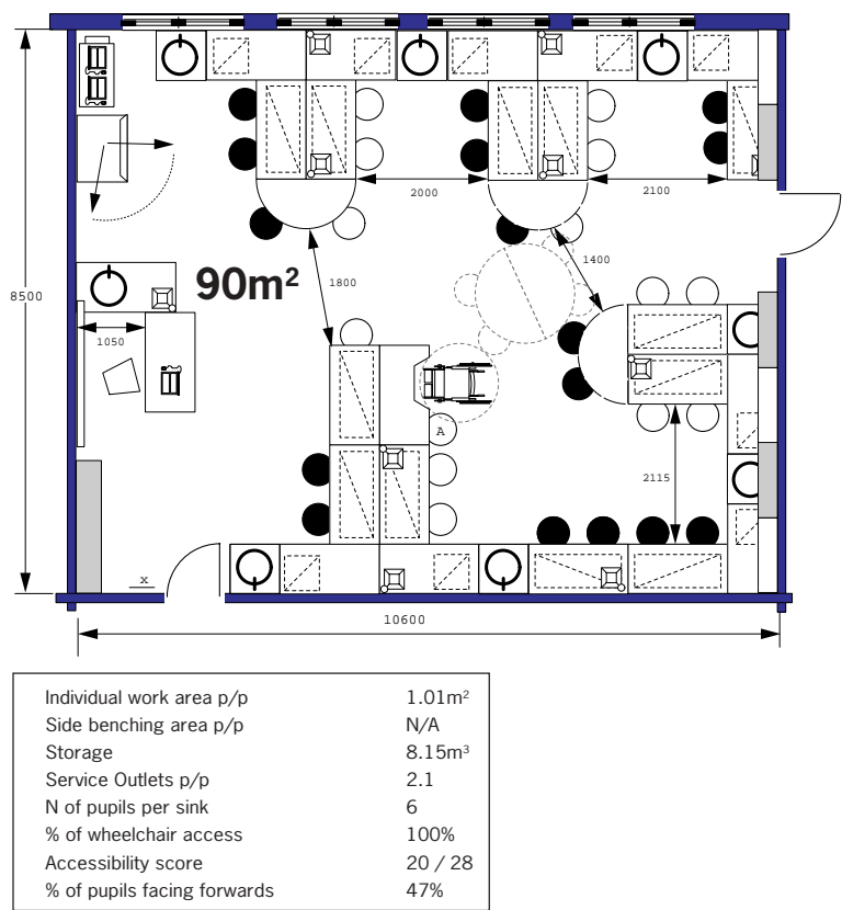
Figure 2/23a: Perimeter Serviced Tables (8.5m).
