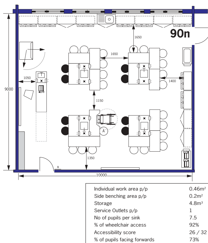
Figure 2/16b: 1200 x 600 Bollard (9m).
