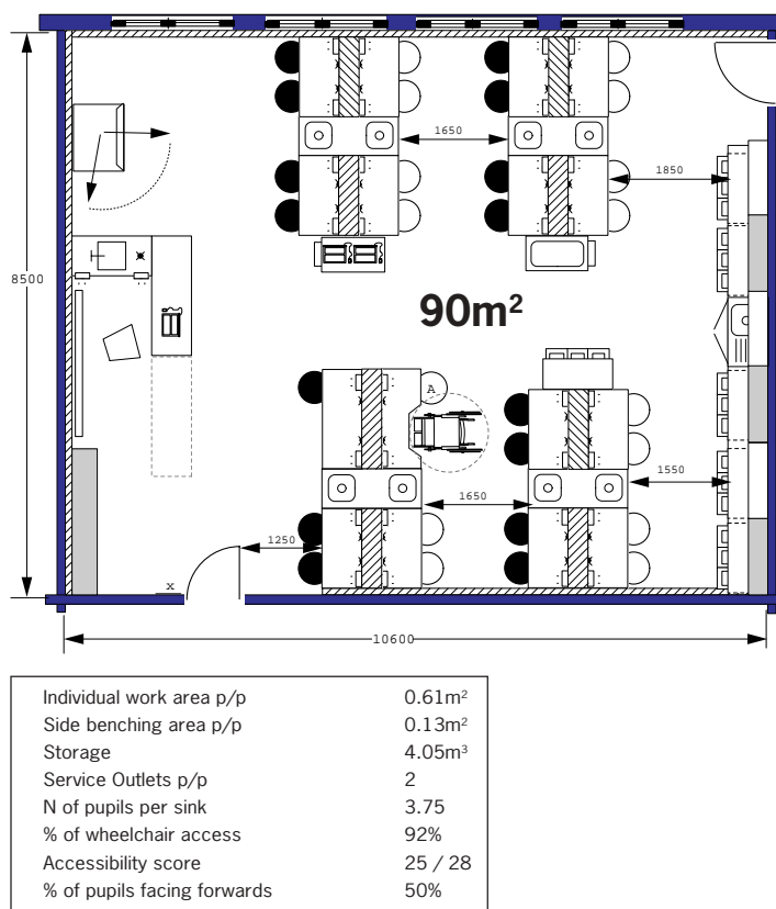
Figure 2/11a: Spine and Island Sink (8.5m).
