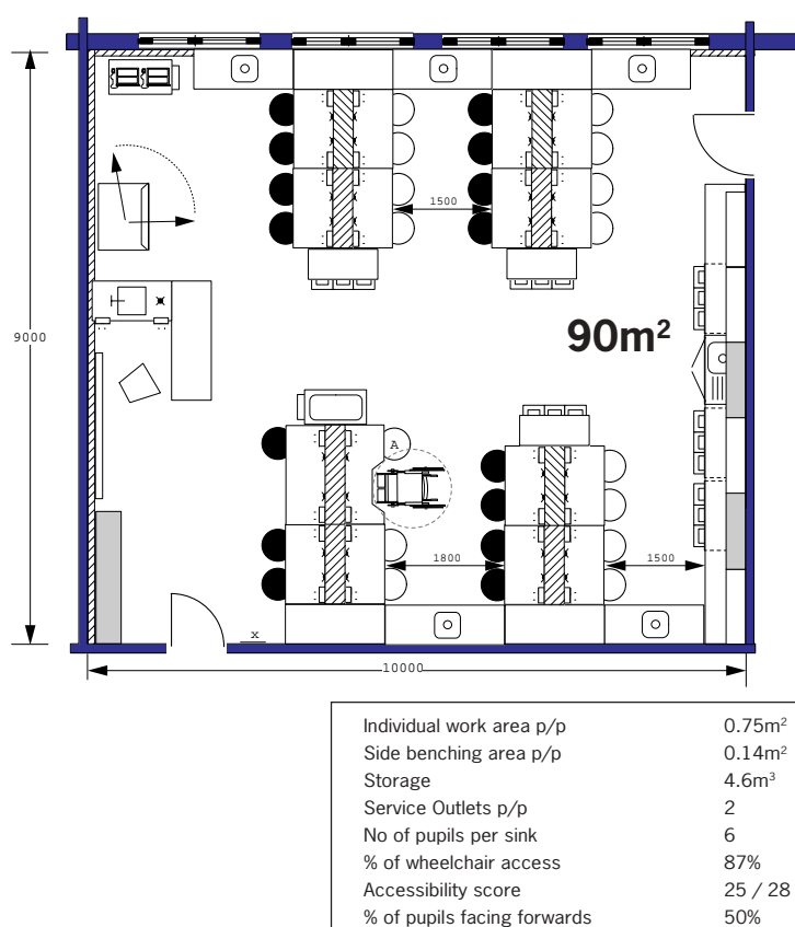
Figure 2/10b: Spine and Perimeter Sink (9m).
